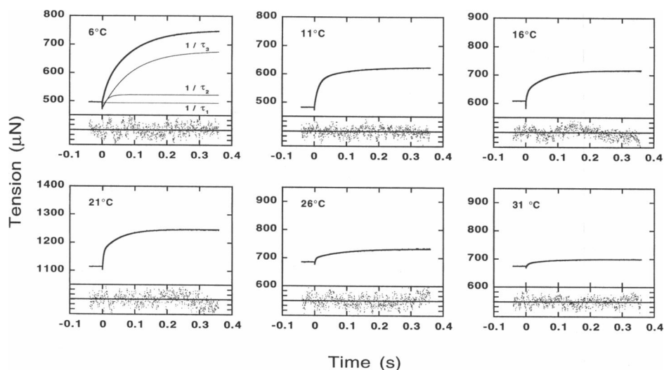
FIGURE 1 T-jump transients of muscle fibers at various temperatures. The response of fibers to a 5°C T-jump is presented. The post-jump temperature is indicated on each panel. Each fiber was activated at 1°C and the temperature was raised to the selected pre-jump temperature in ~35 s immediately before the T-jump. For more details, see Davis and Harrington (1993a). Data were analyzed by nonlinear least-squares fitting to the sum of three exponentials as described in detail in Davis and Harrington (1993a). The best fit line is superimposed on each data set, and residuals of the fit are presented below each data set. The scale of the residuals is \pm 3 \mu\text{N} in each case. Typical resolved exponential components that sum to form the total signal are shown in the 6°C panel. Fiber dimensions were as follows: length = 3.8, 3.9, 4.0, 4.2, 4.0, and 4.2 mm, and cross-sectional area = 8659, 6244, 6128, 10237, 5346, and 5026 \mu\text{m}^2 for 6, 11, 16, 21, 26, and 31°C, respectively. Initial sarcomere spacing was 2.6 \mu\text{m} in each case. Relevant fitted rate constants for 1/\tau_3 are 11.2 (10.9–11.5), 11.7 (11.0–12.5), 15.4 (15.2–15.7), 18.3 (17.8–18.7), 11.2 (10.6–11.9), and 13.6 (11.8–15.6) \text{s}^{-1} for 6, 11, 16, 21, 26, and 31°C, respectively. The values in parentheses represent the 67% joint confidence interval for each parameter.
