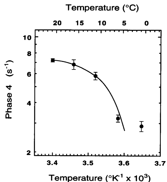
FIGURE 6 Arrhenius plot of the temperature dependence of the Huxley-Simmons phase 4. Note the rise in rate with a plateau at higher temperatures; the datum point at 1°C is not well determined. We subdivide phase 4 into a temperature-sensitive component evident at low temperatures termed phase 4 a and a temperature-insensitive component evident in the plateau region termed phase 4 b . Error bars indicate the standard error of the mean at each point. The number of determinations was n = 13, 18, 13, 16 , and 3 for 1, 6, 11, 16, and 21°C, respectively. The line is a smooth curve drawn through the data.
